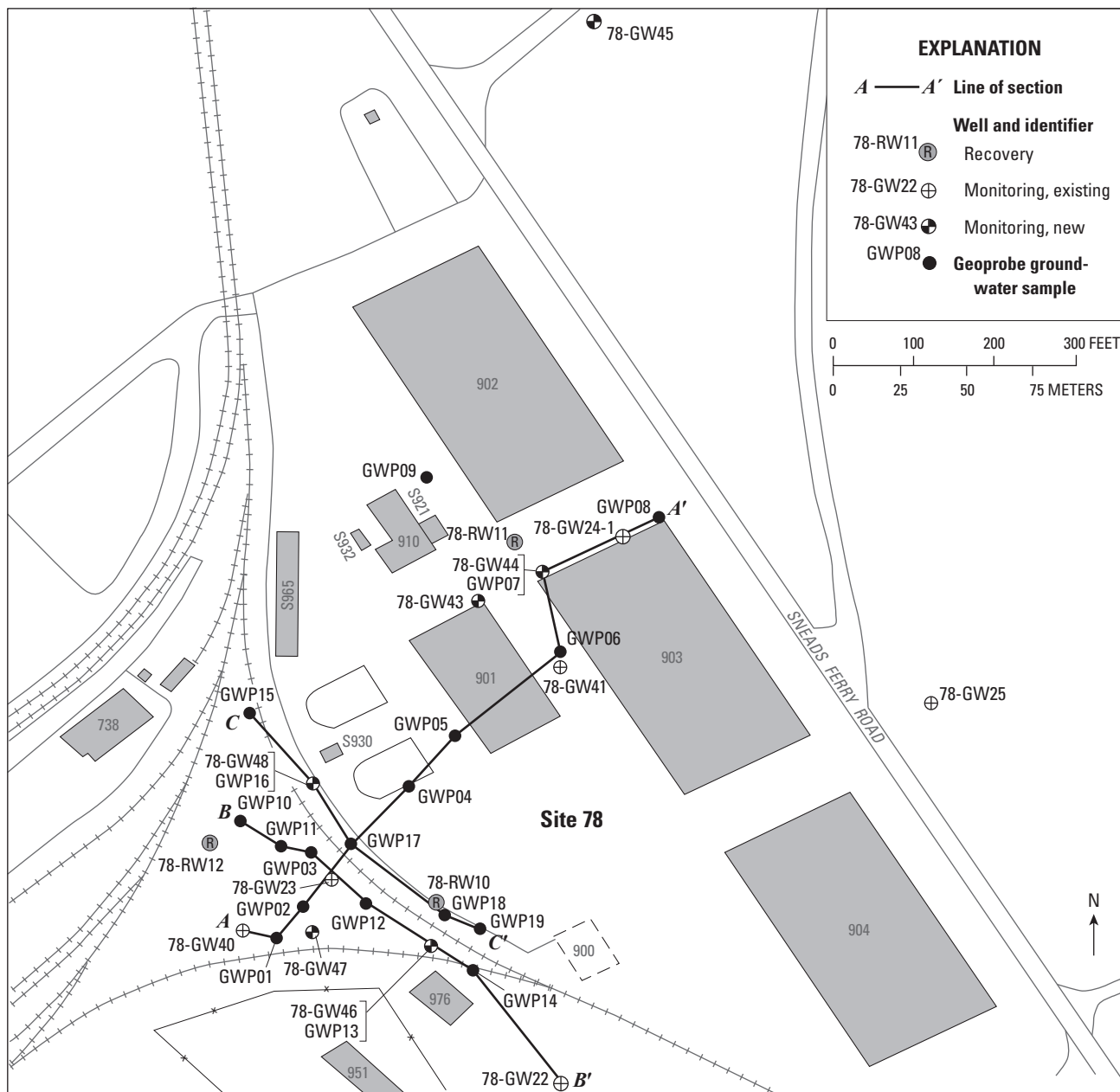
Figure C17. Locations of section lines A–A', B–B', and C–C' at the north contaminated area, Installation Restoration Site 78—Hadnot Point Industrial Area, U.S. Marine Corps Base Camp Lejeune, North Carolina (modified from Baker Environmental Inc., CH2M Hill Federal Group Ltd., and CDM Federal Programs Corp. 2003).
