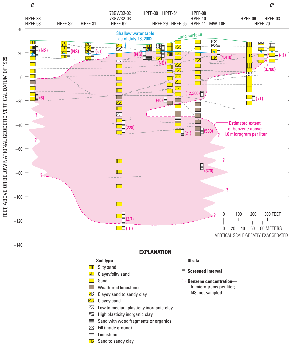
Figure D33. Subsurface distribution of benzene along section C-C' at Underground Storage Tank Program Sites Hadnot Point Fuel Farm and Building 1115 area, March 2002, U.S. Marine Corps Base Camp Lejeune, North Carolina (modified from Catlin Engineers and Scientists 2002c).
