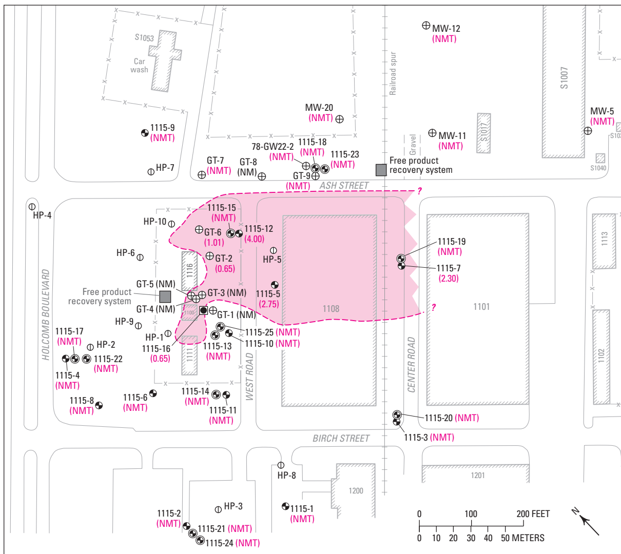
Figure D23. Monitor well and hydropunch locations and occurrence of free-phase hydrocarbon product at Underground Storage Tank Program Site Building 1115, November 1995, U.S. Marine Corps Base Camp Lejeune, North Carolina (modified from Richard Catlin and Associates, Inc. 1998a).
