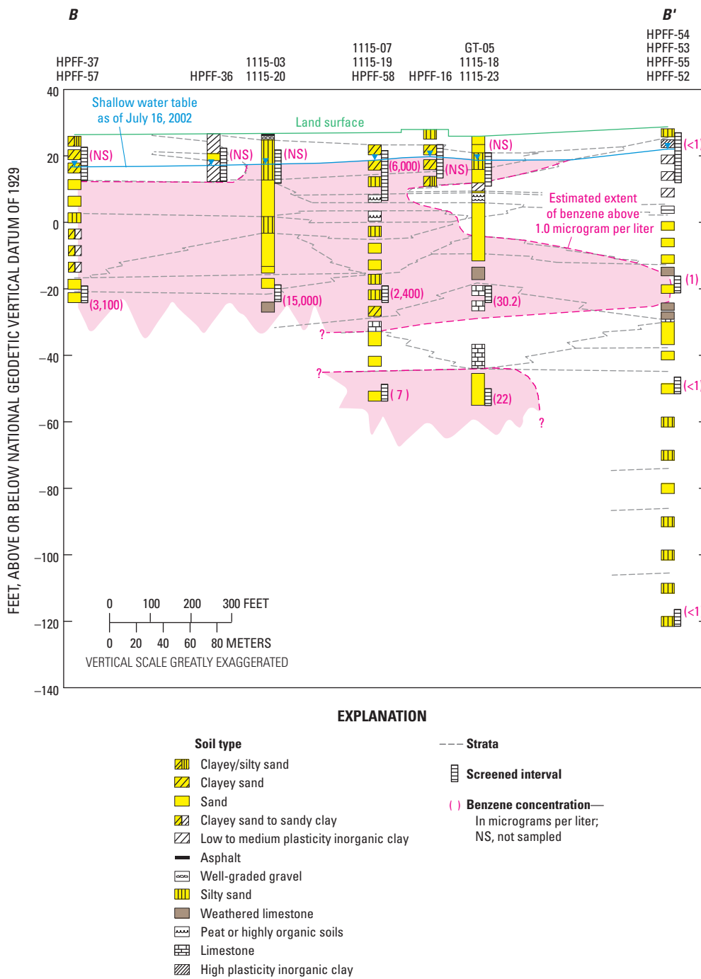
Figure D32. Subsurface distribution of benzene along section B–B' at Underground Storage Tank Program Sites Hadnot Point Fuel Farm and Building 1115 area, February–July 2002, U.S. Marine Corps Base Camp Lejeune, North Carolina (modified from Catlin Engineers and Scientists 2002c).
